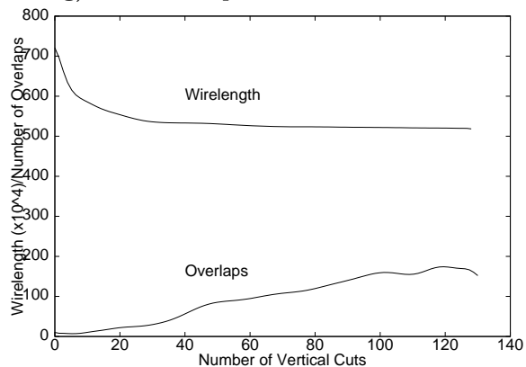
Figure 2: Relationship between number of vertical cuts, total wirelength and number of overlaps. Wirelength is reported in units \times 10^4 .
